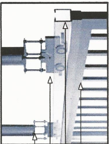
Welded Bottom Member to Track Extruded Track Profile Cantilever Truck Assembly 4" Dia. Galvanized Burried Post
