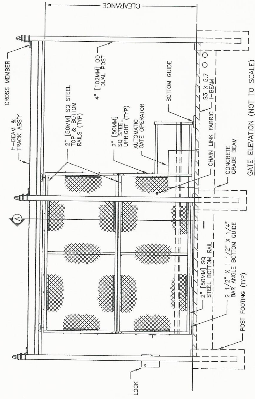
GATE PLAN (NOT TO SCALE)
